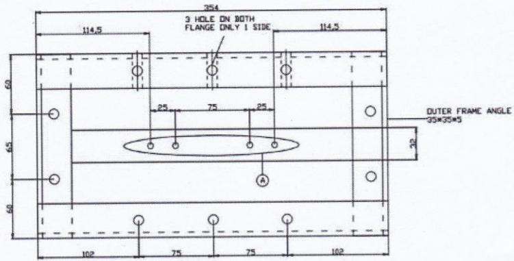
SMALL SIZE CABLE FIXTURE
