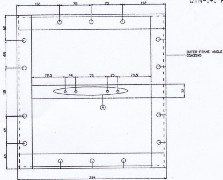
BIG SIZE CABLE FIXTURE
