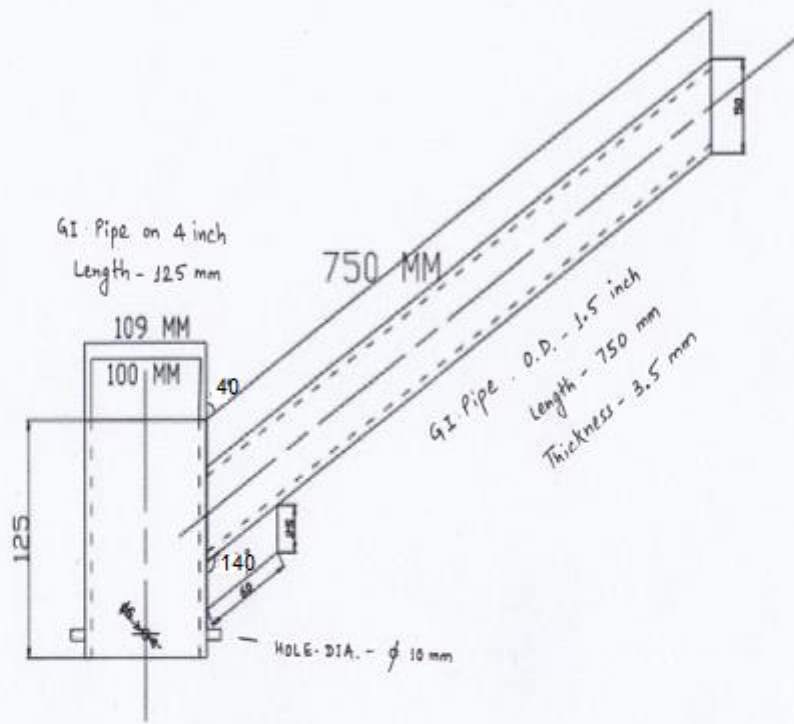
Street Light Bracket
